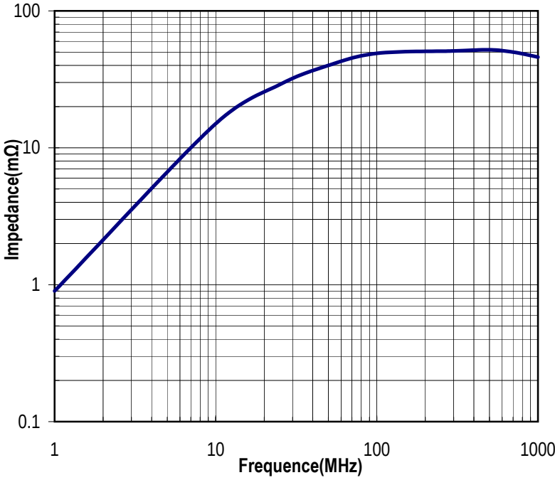
Impedance vs. Frequency Characteristics
